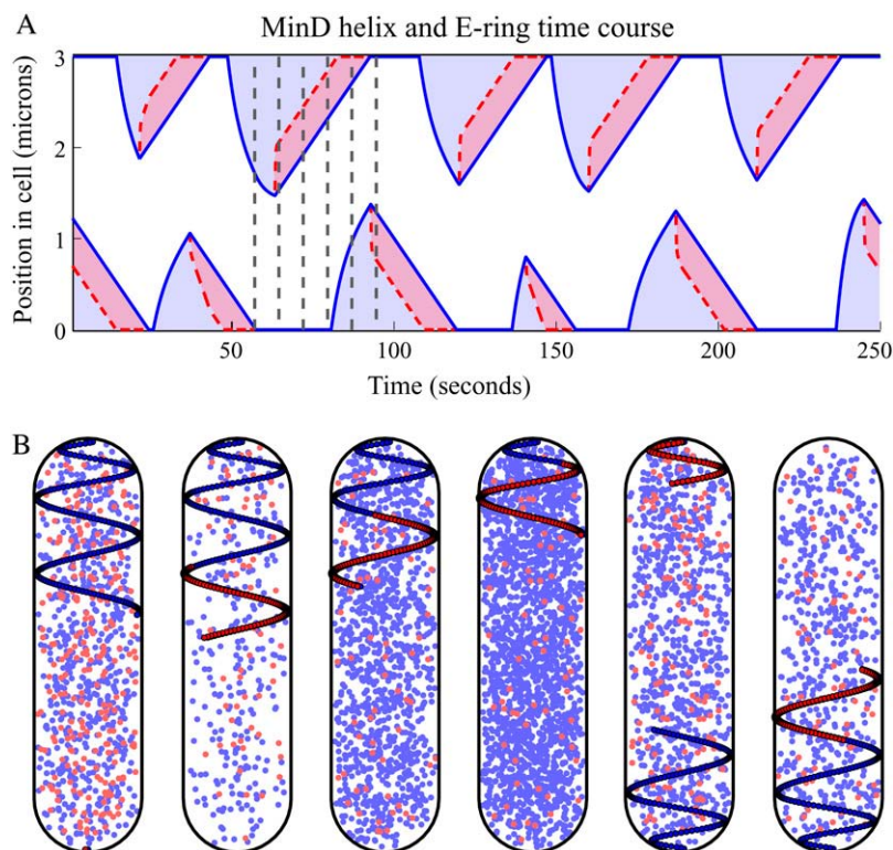
5: A MinD polymer has formed at the bottom and cytosolic MinE dimer concentration has begun to rise. Frame 6: Cytosolic MinE concentration has risen sufficiently to allow an E-ring to form on the lower polymer (equivalent to Frame 2, one half-period later).
