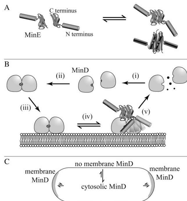
FIGURE 1 Proposed dimer model. (A) MinE undergoes dimerization. The N-terminus anti-MinD domain is involved in inducing hydrolysis by MinD and the C-terminus is involved in dimerization and E-ring formation. Residues 45 and 49, involved in E-ring formation, are shown as light patches on the underside of the MinE dimer. (B) MinD cycles from the cytosol where it binds ATP (i), dimerizes (ii), attaches to the membrane (iii), recruits MinE (iv), hydrolyzes ATP, and is released from the membrane (v). MinE is proposed to undergo a conformation change in which the anti-MinD domain moves to the MinD dimerization face (v) simultaneously blocking polymerization of dimers and inducing MinD ATPase activity. (C) If MinD attaches at the poles, hydrolysis and release is assumed to be slower leading to an accumulation of dimers at the pole.
